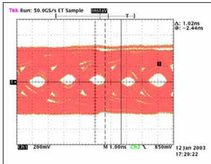
Figure 5b. Eye Diagram with 100ft Cables 100ft, 520Mbps, t_{TJ}=1020ps , t_{MJ} = N/A , 1.87 \cdot 10^{13} bits transmitted. No errors. Vertical scale: 200mV/Div. Horizontal scale: 1ns/Div.
