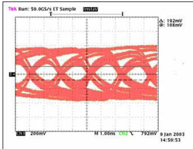
Figure 5a. Eye Diagram with 100ft Cables 100ft, 480Mbps, t_{TJ}=660ps , t_{MJ} = N/A , 1.73 \cdot 10^{13} bits transmitted. No errors. Vertical scale: 200mV/Div. Horizontal scale: 1ns/Div.
